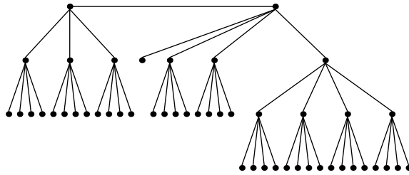
Festoon Tree for d = 4, n = 49
