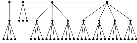
Festoon Tree for d = 4, n = 47
