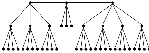
Festoon Tree for d = 4, n = 41
