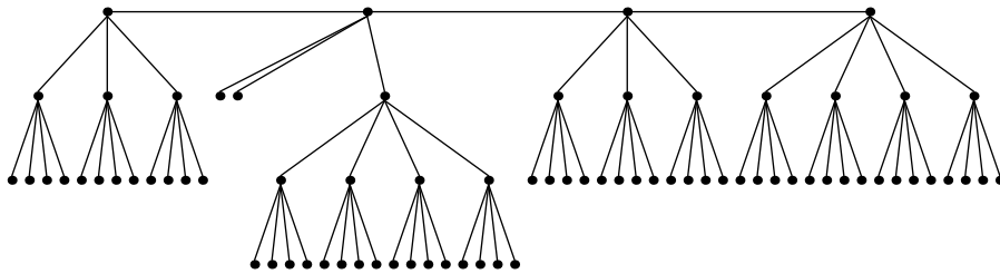
Festoon Tree for d = 4, n = 77
