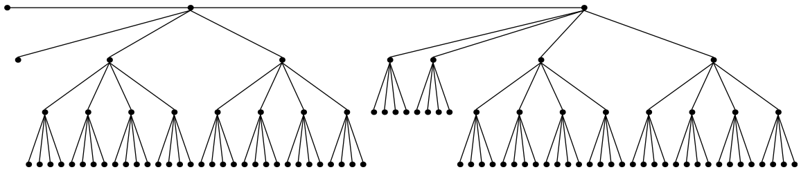
Festoon Tree for d = 4, n = 98
