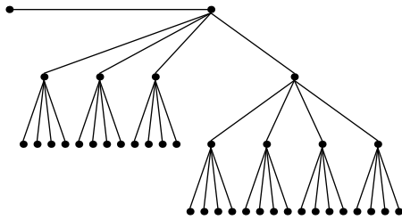
Festoon Tree for d = 4, n = 38
