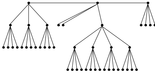
Festoon Tree for d = 4, n = 45
