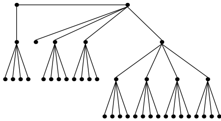
Festoon Tree for d = 4, n = 39
