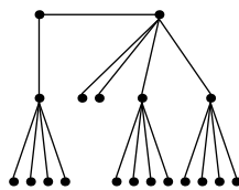
Festoon Tree for d = 4, n = 19
