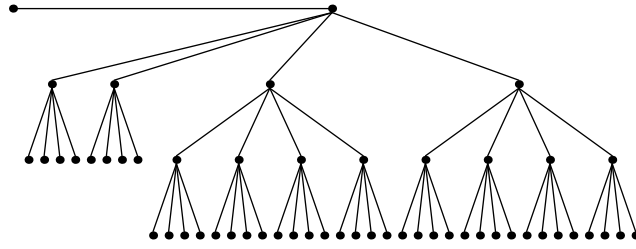
Festoon Tree for d = 4, n = 54
