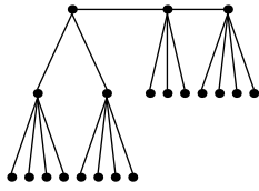
Festoon Tree for d = 4, n = 20
