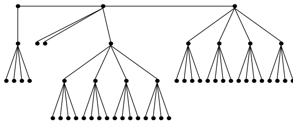
Festoon Tree for d = 4, n = 51
