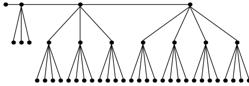
Festoon Tree for d = 4, n = 42
