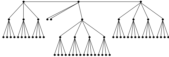
Festoon Tree for d = 4, n = 61
