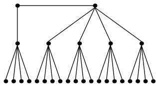
Festoon Tree for d = 4, n = 27
