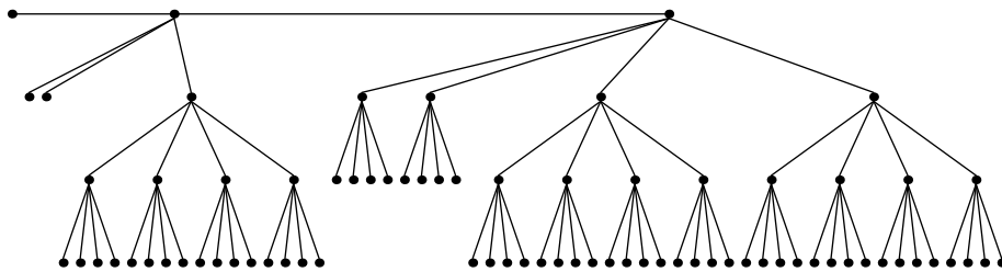
Festoon Tree for d = 4, n = 78
