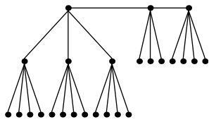
Festoon Tree for d = 4, n = 25
