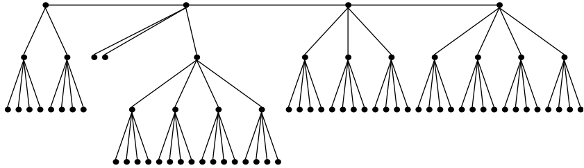
Festoon Tree for d = 4, n = 72
