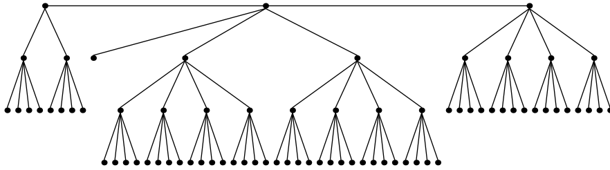
Festoon Tree for d = 4, n = 76
