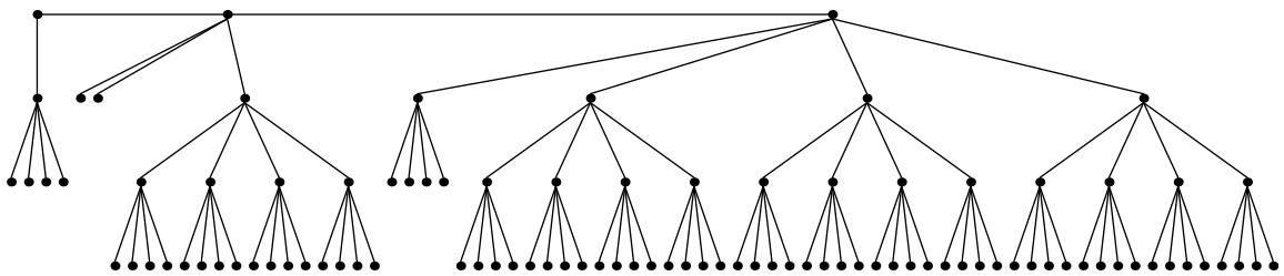
Festoon Tree for d = 4, n = 99
