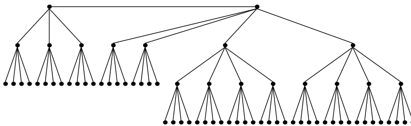
Festoon Tree for d = 4, n = 69
