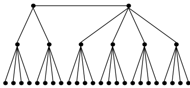
Festoon Tree for d = 4, n = 32
