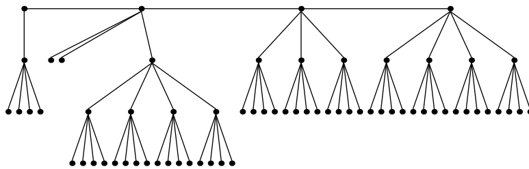
Festoon Tree for d = 4, n = 67
