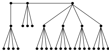
Festoon Tree for d = 4, n = 31
