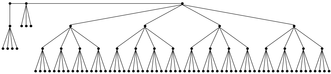
Festoon Tree for d = 4, n = 95
