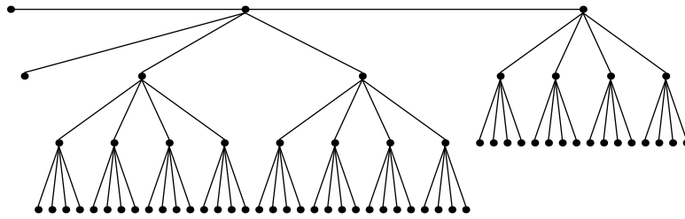
Festoon Tree for d = 4, n = 66
