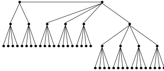
Festoon Tree for d = 4, n = 48
