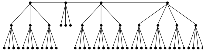
Festoon Tree for d = 4, n = 57
