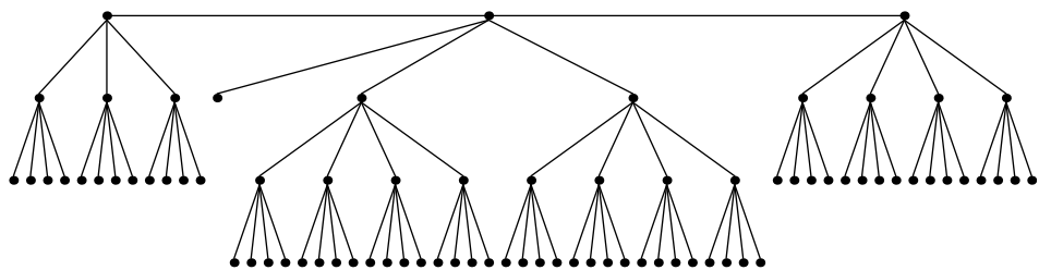
Festoon Tree for d = 4, n = 81
