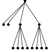
Festoon Tree for d = 4, n = 13
