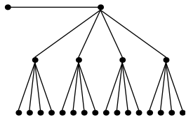
Festoon Tree for d = 4, n = 22
