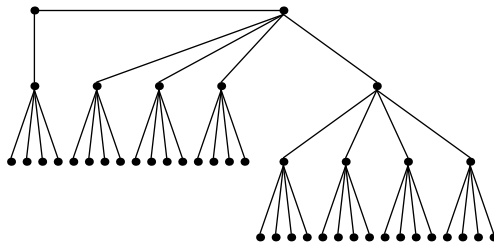
Festoon Tree for d = 4, n = 43
