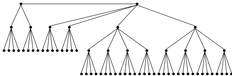
Festoon Tree for d = 4, n = 63
