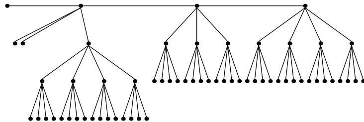
Festoon Tree for d = 4, n = 62
