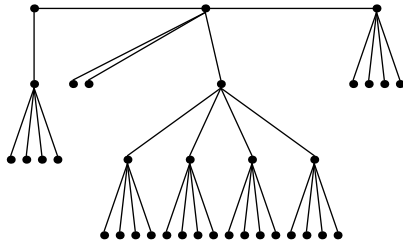
Festoon Tree for d = 4, n = 35
