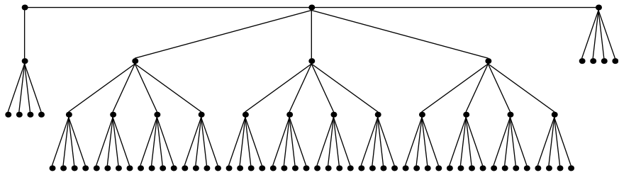
Festoon Tree for d = 4, n = 74
