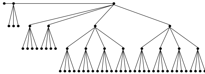
Festoon Tree for d = 4, n = 58
