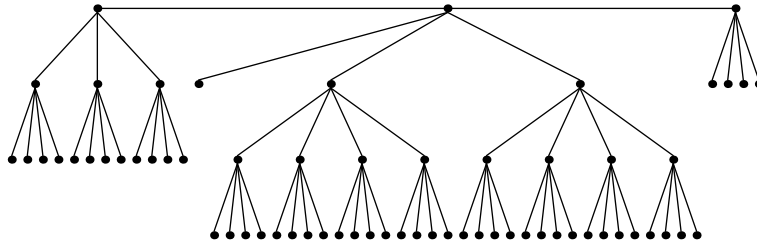
Festoon Tree for d = 4, n = 65
