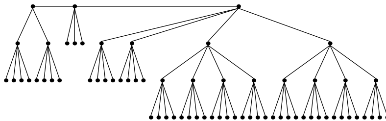
Festoon Tree for d = 4, n = 68
