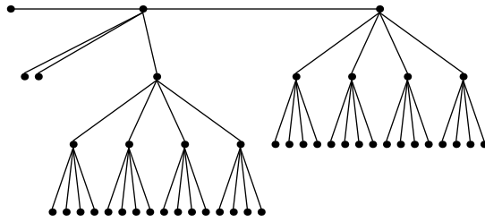
Festoon Tree for d = 4, n = 46
