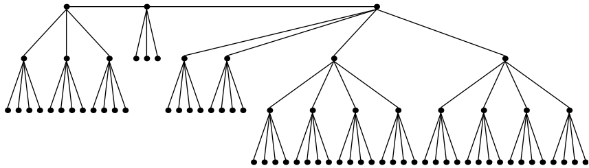
Festoon Tree for d = 4, n = 73
