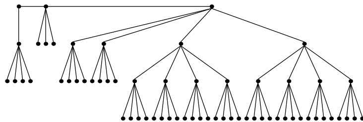
Festoon Tree for d = 4, n = 63
