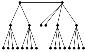
Festoon Tree for d = 4, n = 24
