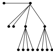
Festoon Tree for d = 4, n = 14
