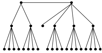
Festoon Tree for d = 4, n = 28
