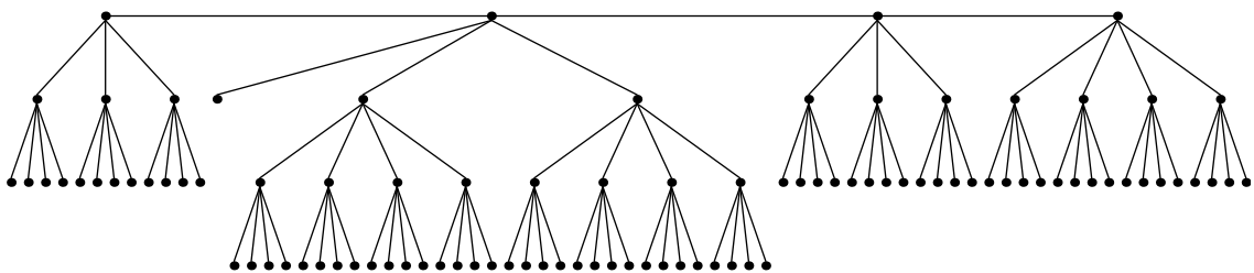
Festoon Tree for d = 4, n = 96
