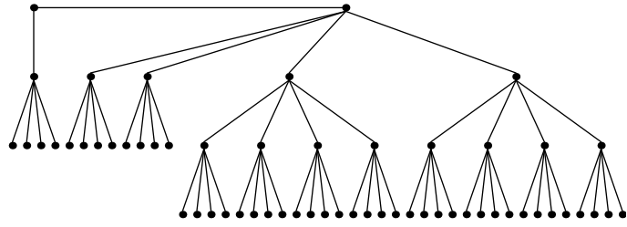
Festoon Tree for d = 4, n = 59
