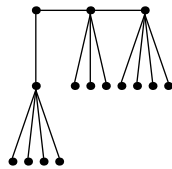
Festoon Tree for d = 4, n = 15
